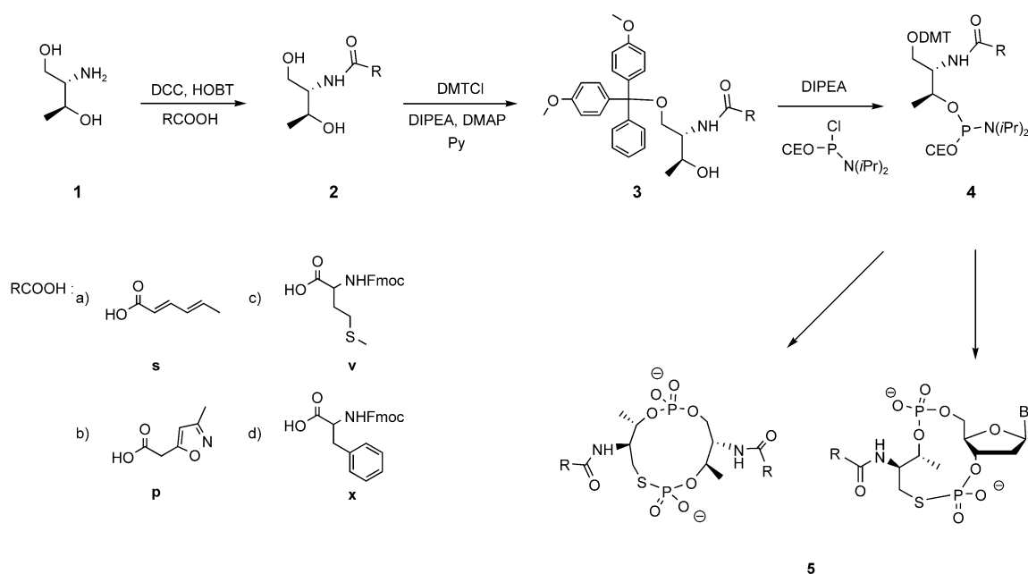
Scheme 2. Synthesis of cyclic DNA hybrids.
